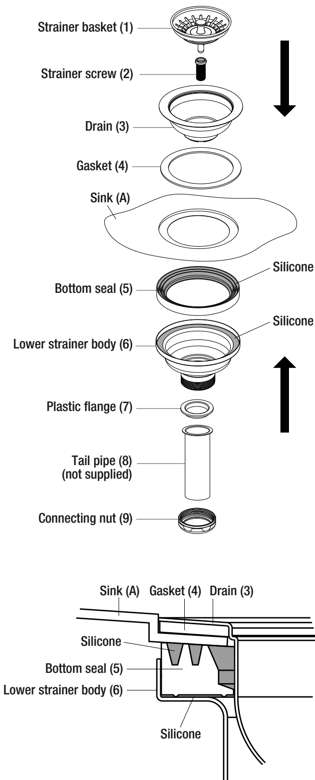
DRAIN INSTALLATION DETAIL
