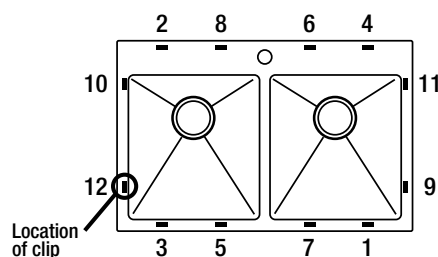
Tightening sequence for clips
