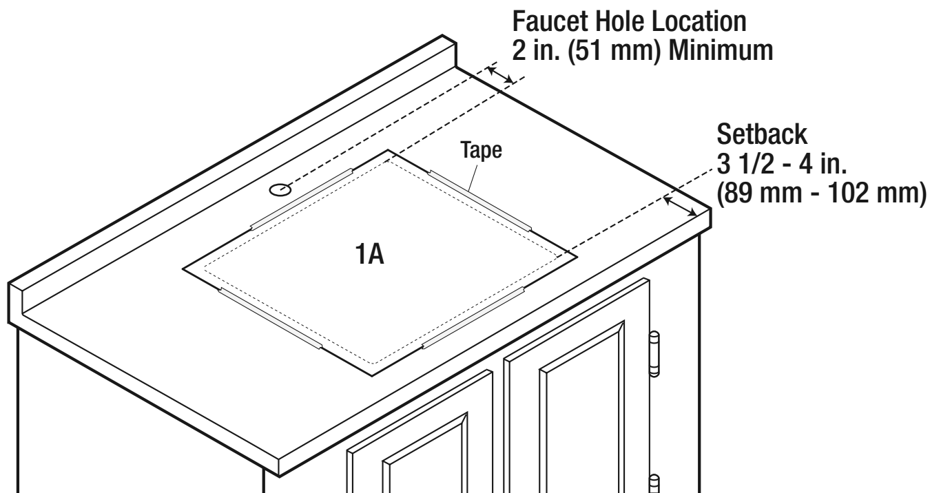
Undermount installation
