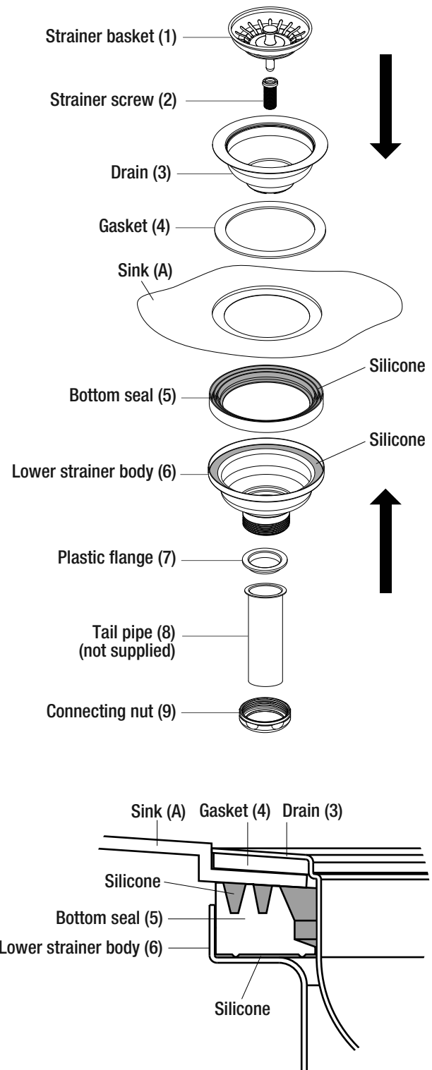
DRAIN INSTALLATION DETAIL
