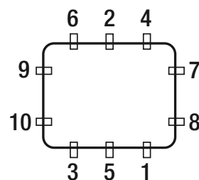
Tightening sequence for clips
