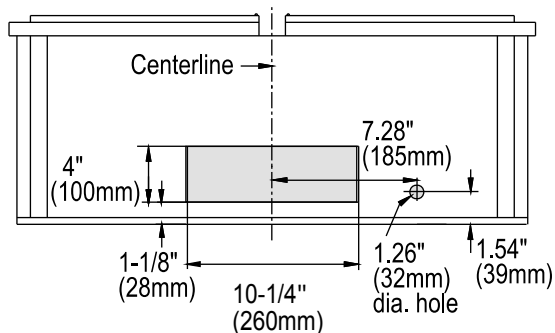
Top Venting Option
